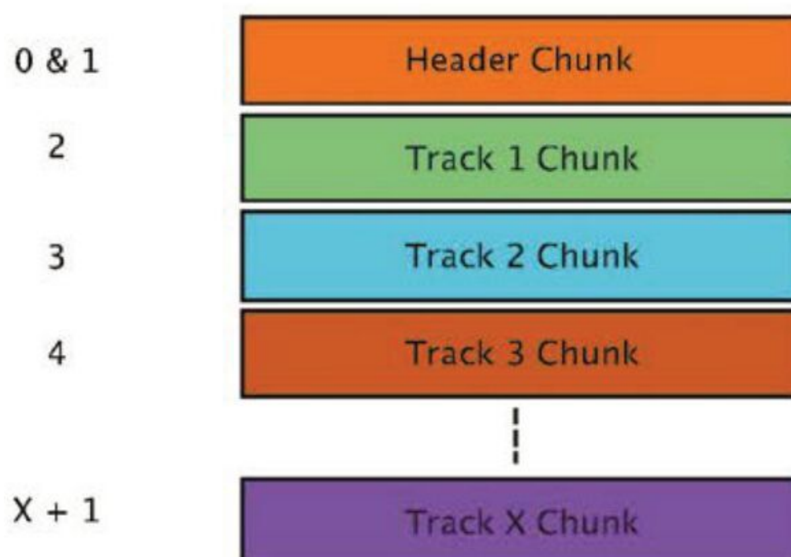
Chunk Number Standard MIDI File format
