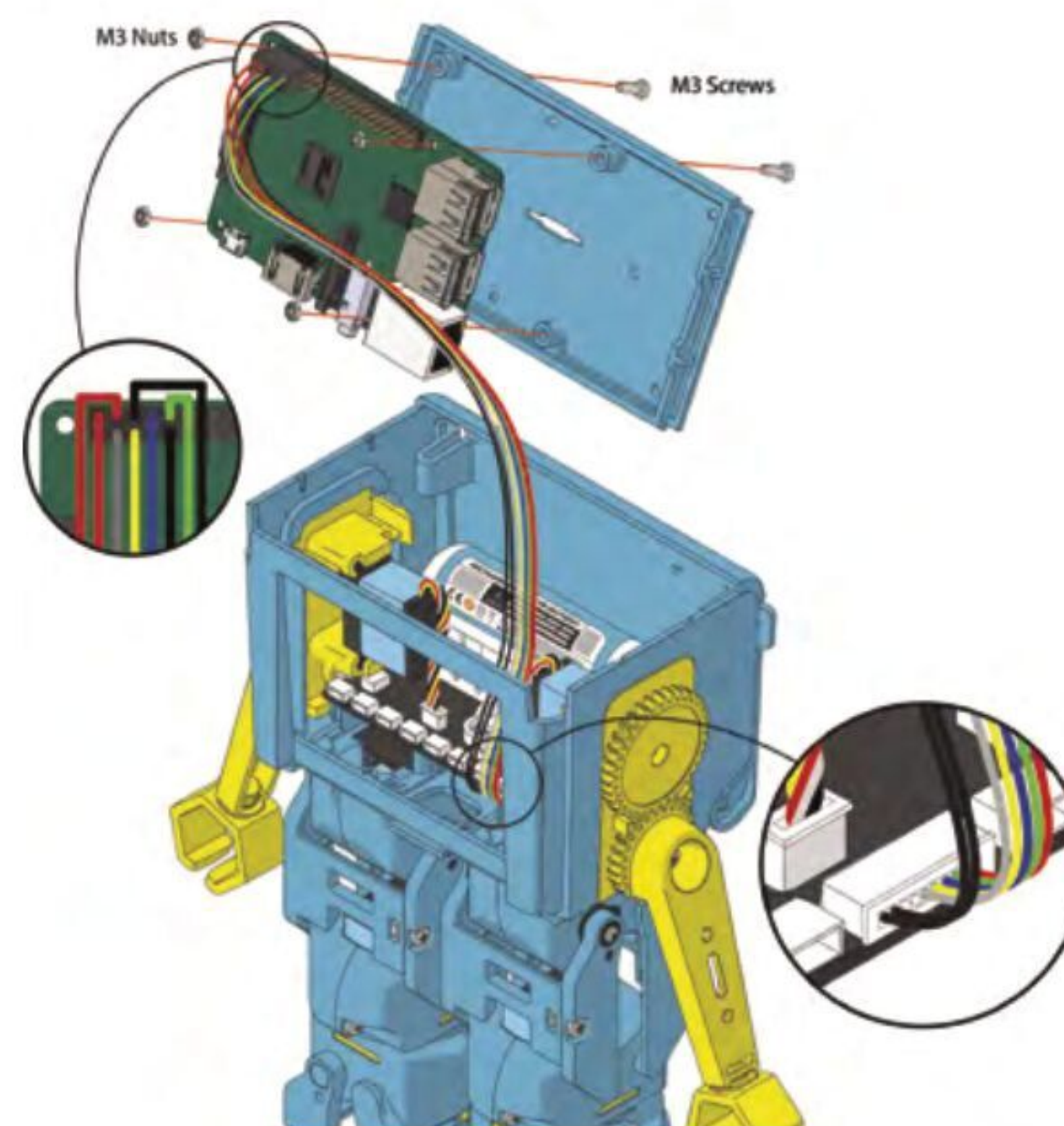
▼ Fitting Raspberry Pi inside Marty V2
