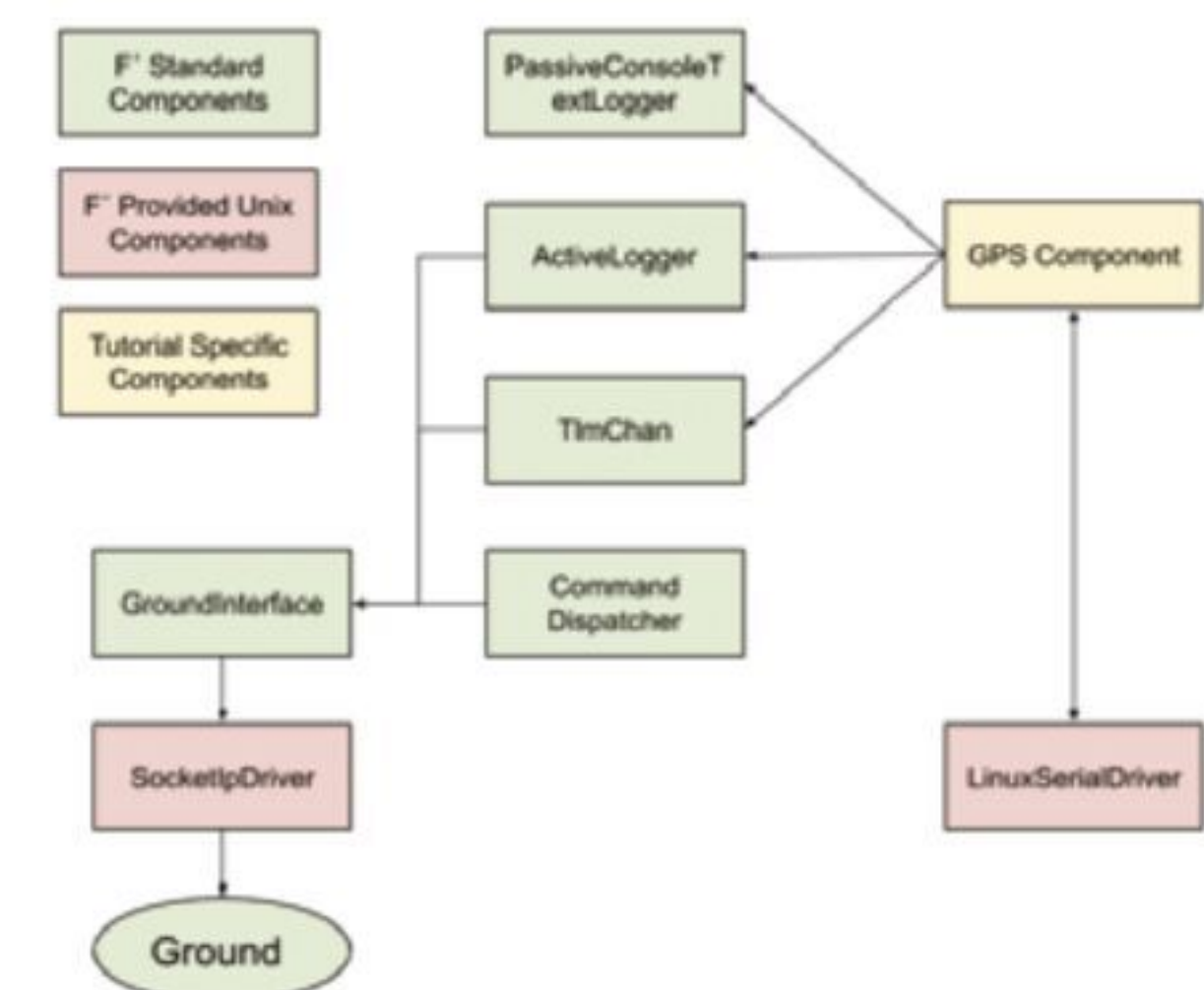
F' GPS Application Diagram - v0.1
