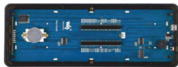
▲ A Raspberry Pi Pico flashed with the software can be slotted into the clock's rear female headers
