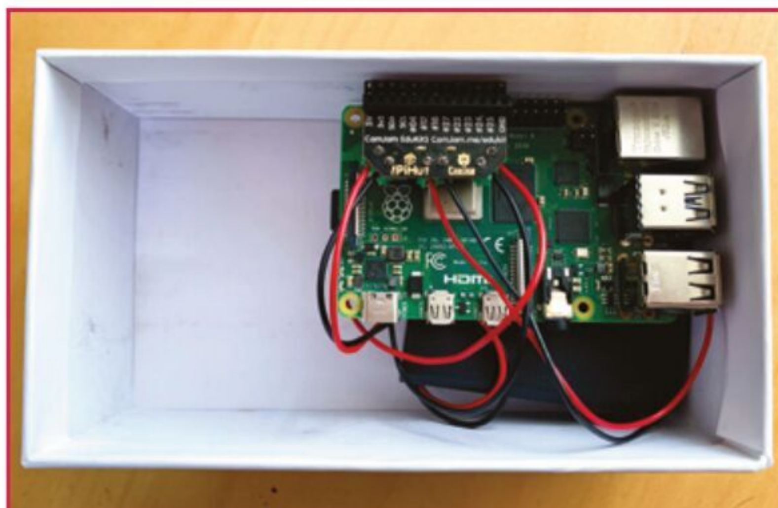
▲ You can use the battery pack and Raspberry Pi 4 as 'ballast' at the rear. Add a power bank for true remote computing!
