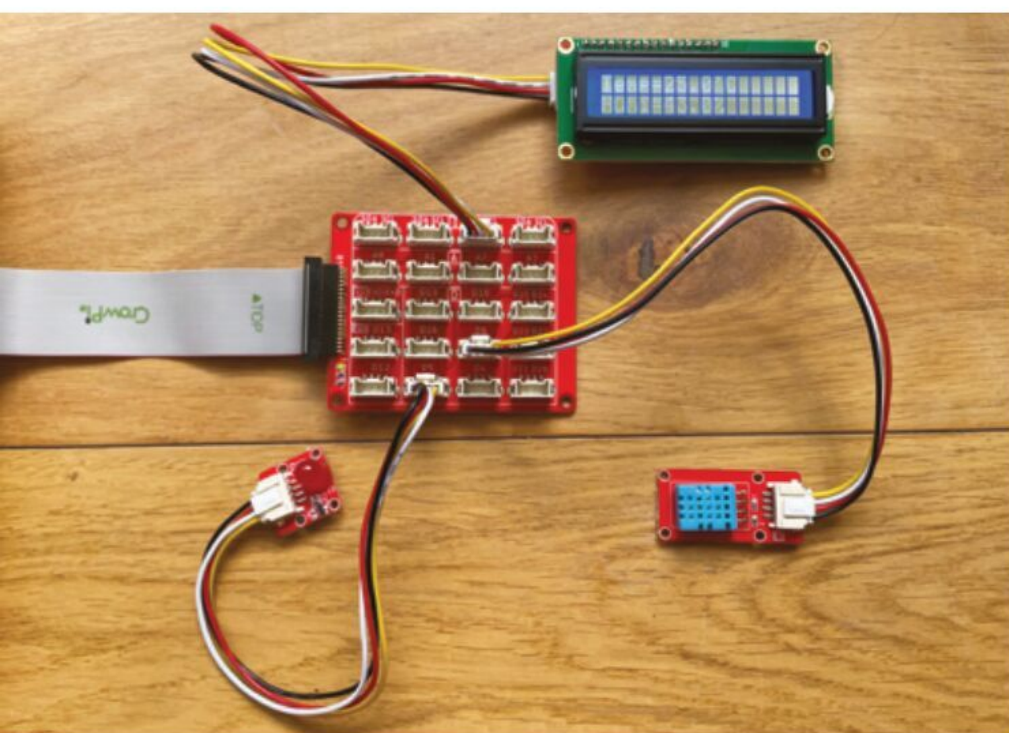
▲ The CrowPi L Base Shield is connected for electronic prototyping
