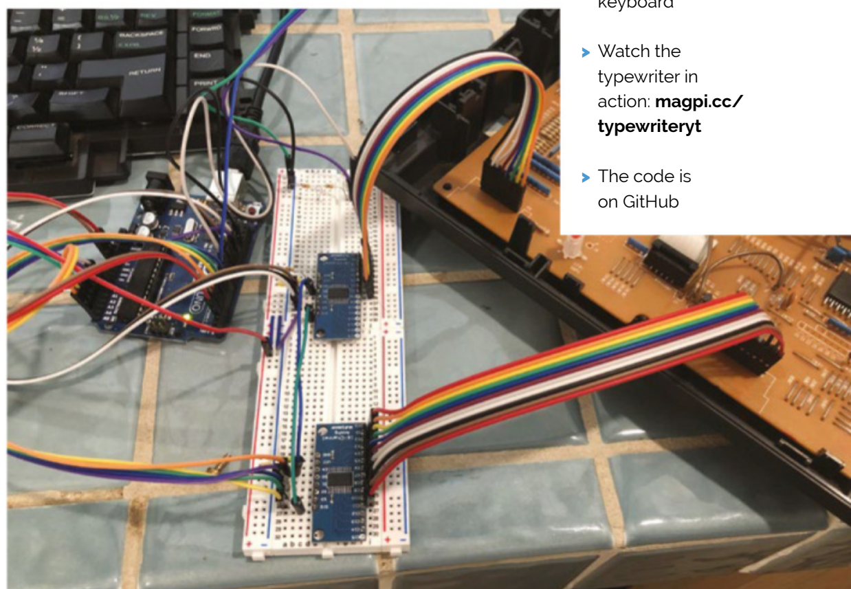
▲ A voltage divider circuit has been created so that the 5V output of the Arduino is at a safe 3.3V level for Raspberry Pi
