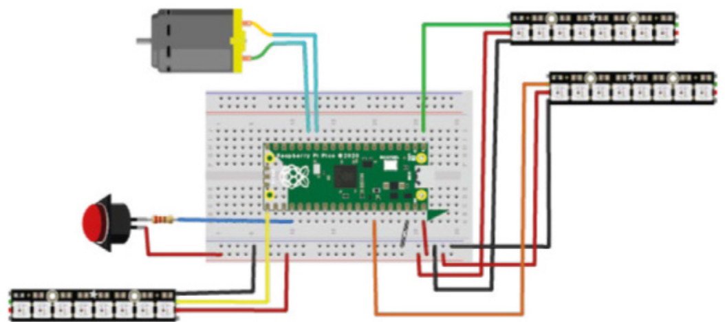
▲ Figure 1 The components are arranged in sections to make separation easier. Bottom left is the handle, bottom right is the tank, top right is the wheels, and then the motor is on its own
