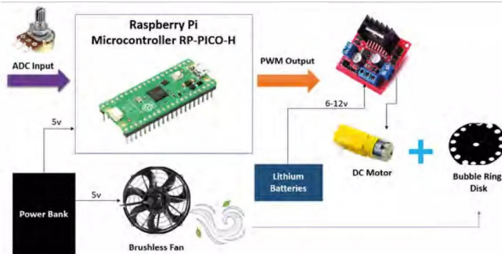
DIY Bubble Machine Block Diagram
