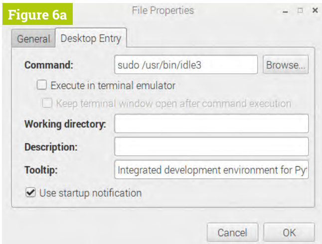
▲ Figure 6 Changing the command so that IDLE or Thonny will run in supervisor mode
