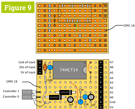
▲ Figure 9 Layout of the LED driver and signal conditioner board
