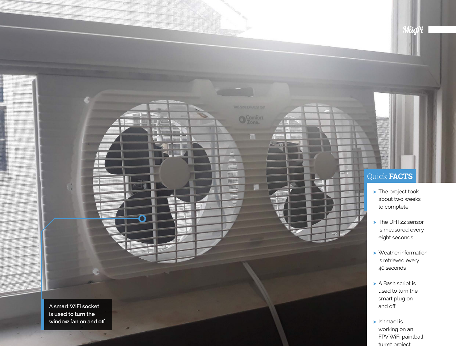
The indoor temperature is read by a DHT22 sensor; if it's cooler outside, the fan is turned on
