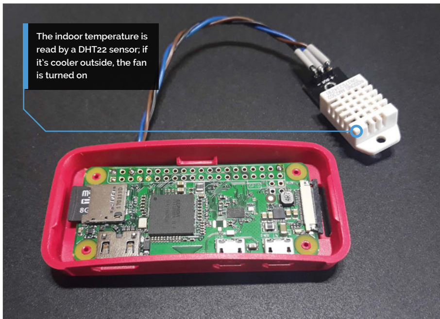
▲ The DHT22 sensor is connected to power, ground, and GPIO 4 pins on a Raspberry Pi Zero – a 10kΩ resistor is recommended
