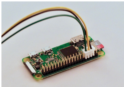
▲ Luckily, the printer's connector matches up with the GPIO pins and can be directly attached
