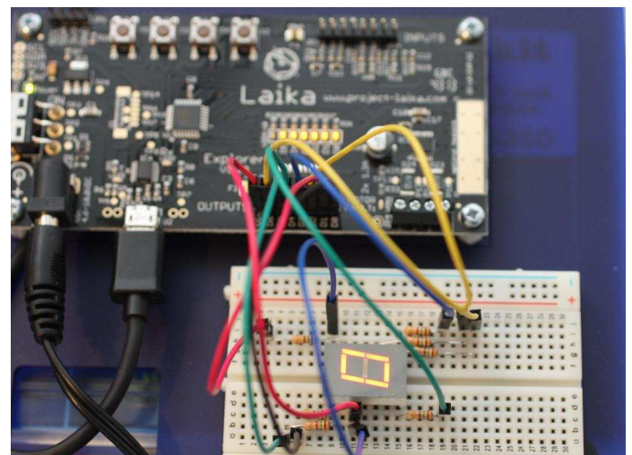
Figure 7.0 – 7-segment control
