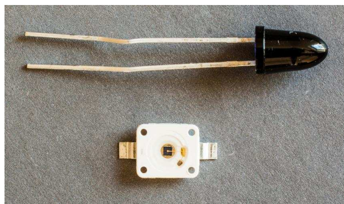
Figure 3 – Infrared Emitters – Top: SFH4545, Bottom: SFH4233
