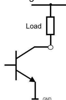
Figure 3.0 - Transistor switch
