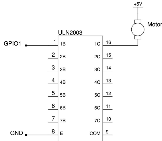
Figure 2 - ULN2003 and small DC motor
