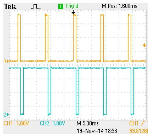
Figure 1 - Pulse width modulation signals
