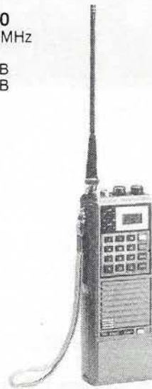
◀ TR 3500 FM 430 - 440 MHz 1,5 W/300 MW 0,3 \mu V = 25 dB 1,0 \mu V = 35 dB
