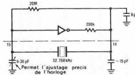
Figure 2. Crystal Oscillator
