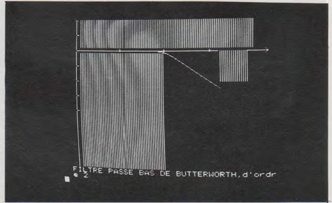
PREMIER EXEMPLE: BUTTERWORTH ORDRE 2 f_0 = 1 \text{ kHz} f_1 = 20 \text{ kHz} A = 40 \text{ db}
