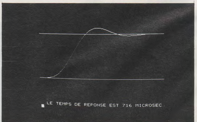
QUATRIEME EXEMPLE: BUTTERWORTH ORDRE 5 f_0 = 1 \text{ kHz} f_1 = 20 \text{ kHz} A = 40 \text{ db}
