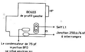
Figure 4 Modification BFO.
