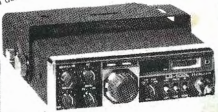
▲ Prix : 4765 F LS 102X Transceiver 28 MHz tous modes USB/LSB/CW/FM/AM, 10 W, 12 W, affichage digital.
