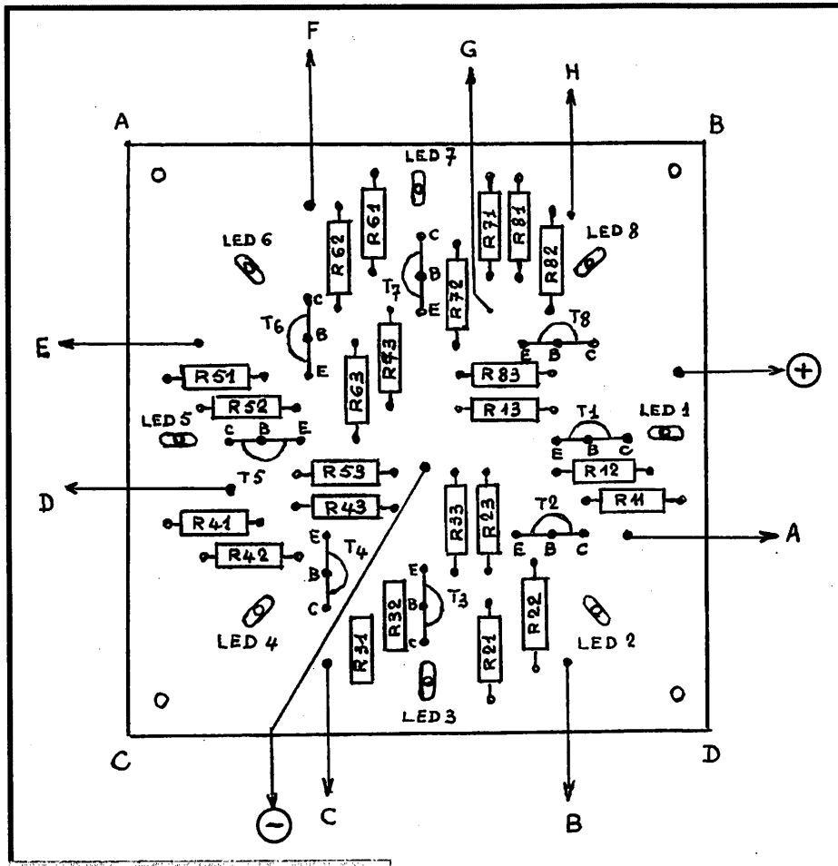
Figure 6. Circuit amplificateur.
