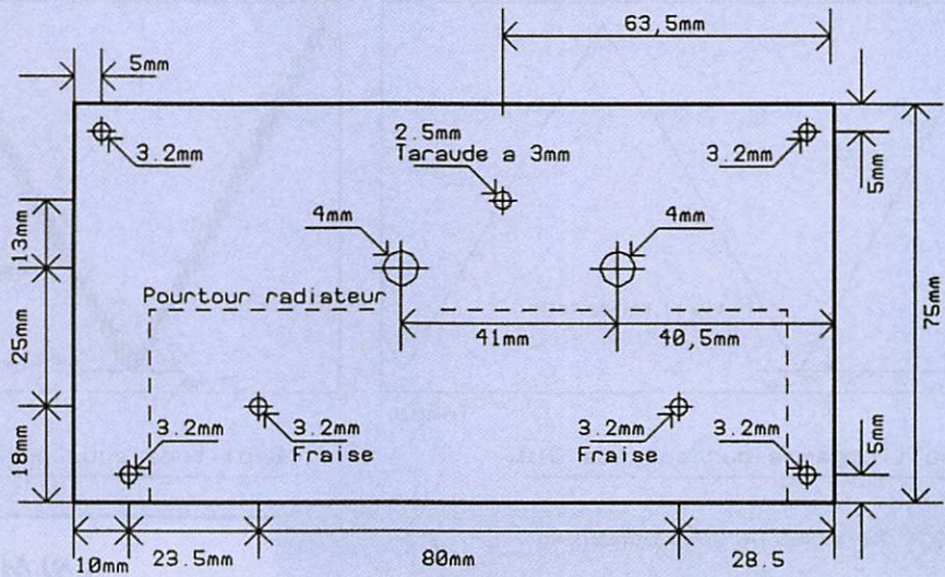
PLAQUE ALUMINIUM Epaisseur: 3.5mm a 4mm
