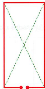
Configuration "x" haute Type Bird Cage (G4ZU)
