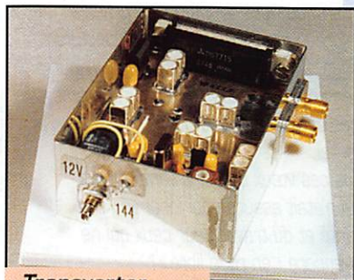
Transverter DB6NT.
