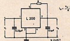
Fig. 2 - Programmable current regulator
