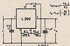
Fig. 1 - Programmable voltage regulator with current limiting
