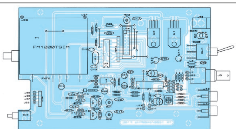
Implantation.
