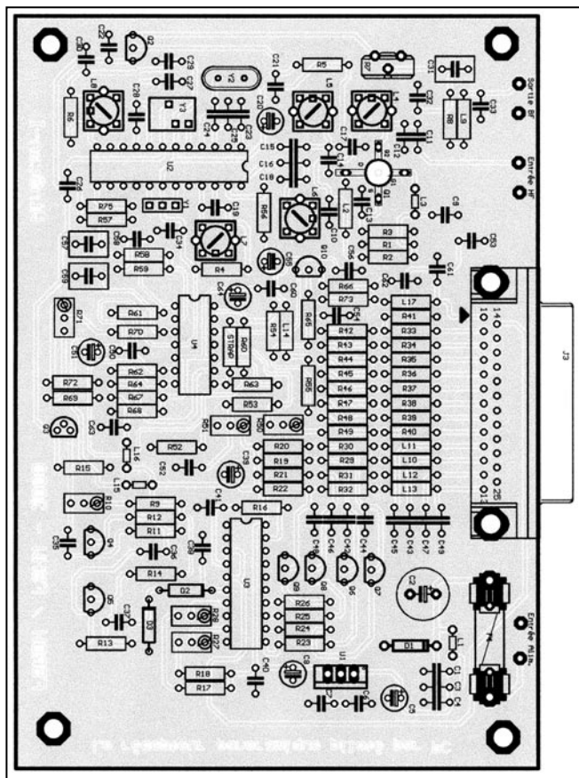
Implantation.
