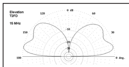
Figure 4: Élévation T2FD.
