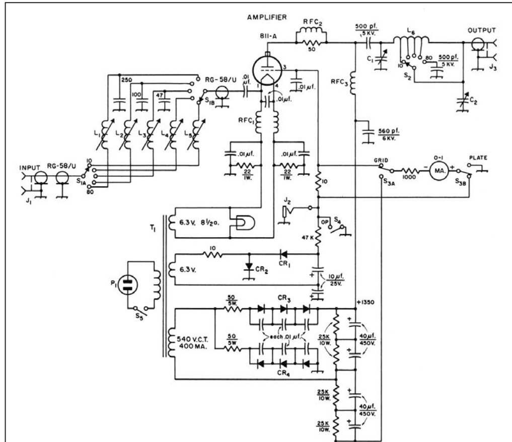
Circuit diagram of the 200-watt grounded-grid linear amplifier.
