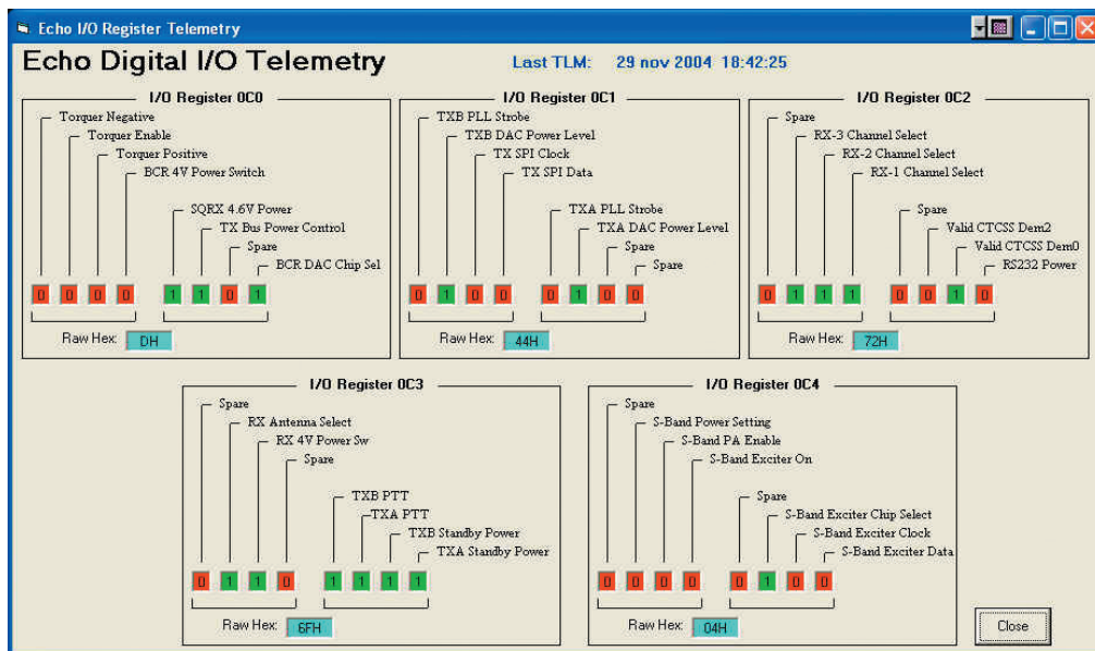
Figure 11: Registres I/O.
