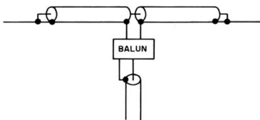
Fig 5—The double bazooka, sometimes called a coaxial dipole. The antenna is self-resonant at 3.75 MHz. The resonator stubs are 43.23-ft lengths of RG-58A coax.
