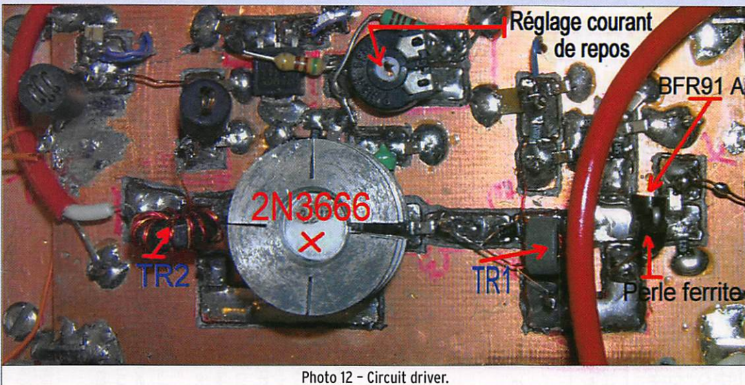
Photo 12 - Circuit driver.
